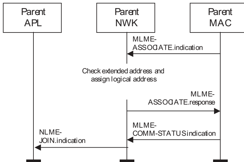
25 26 27 28 29 30 31 32 33 34 35 36 37 38 39 40 41 42 43 Figure 50 Procedure for handling a join request
